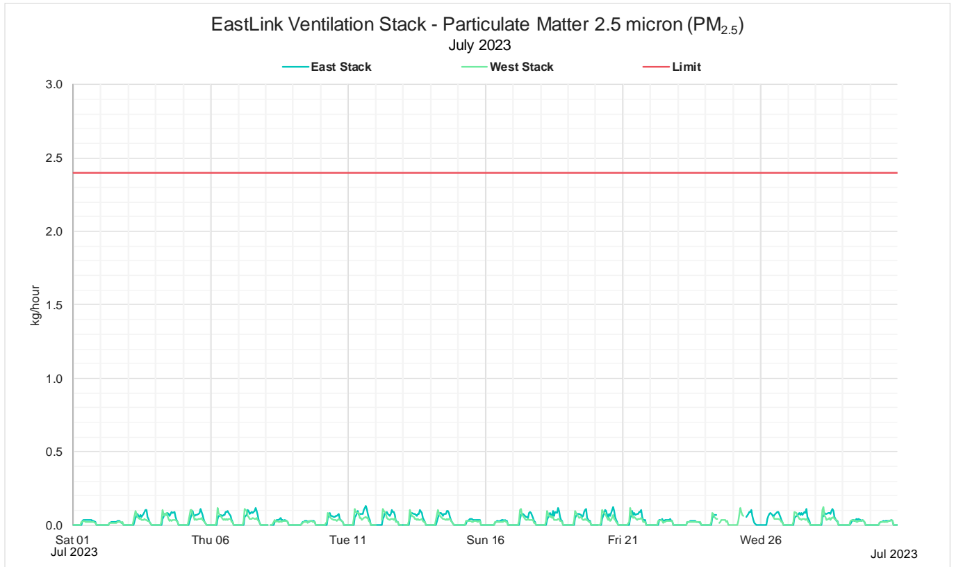
Figure 5: July 2023 Monthly 1 hour mass rate PM 2.5
