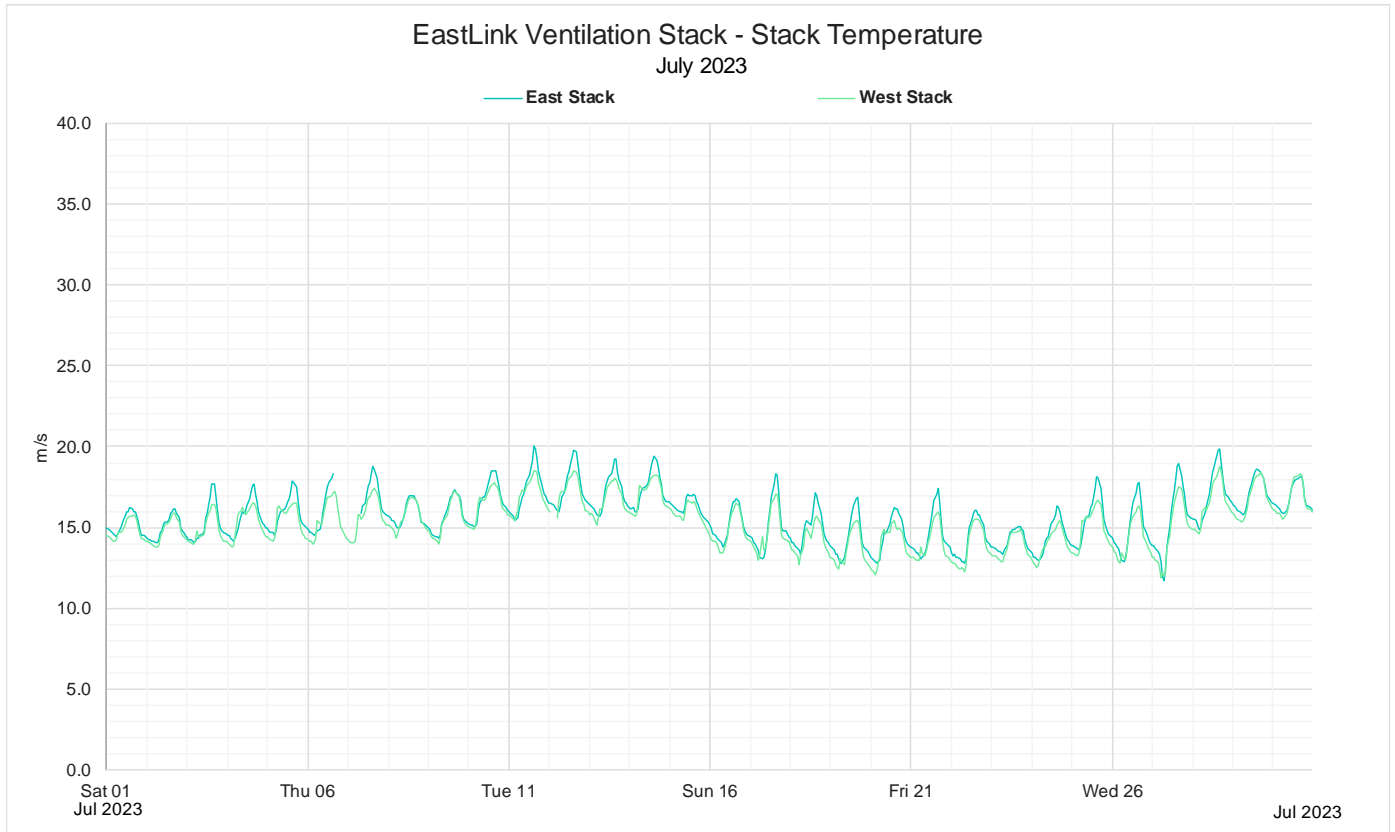
Figure 8: July 2023 Monthly 1 hour average stack temperature
