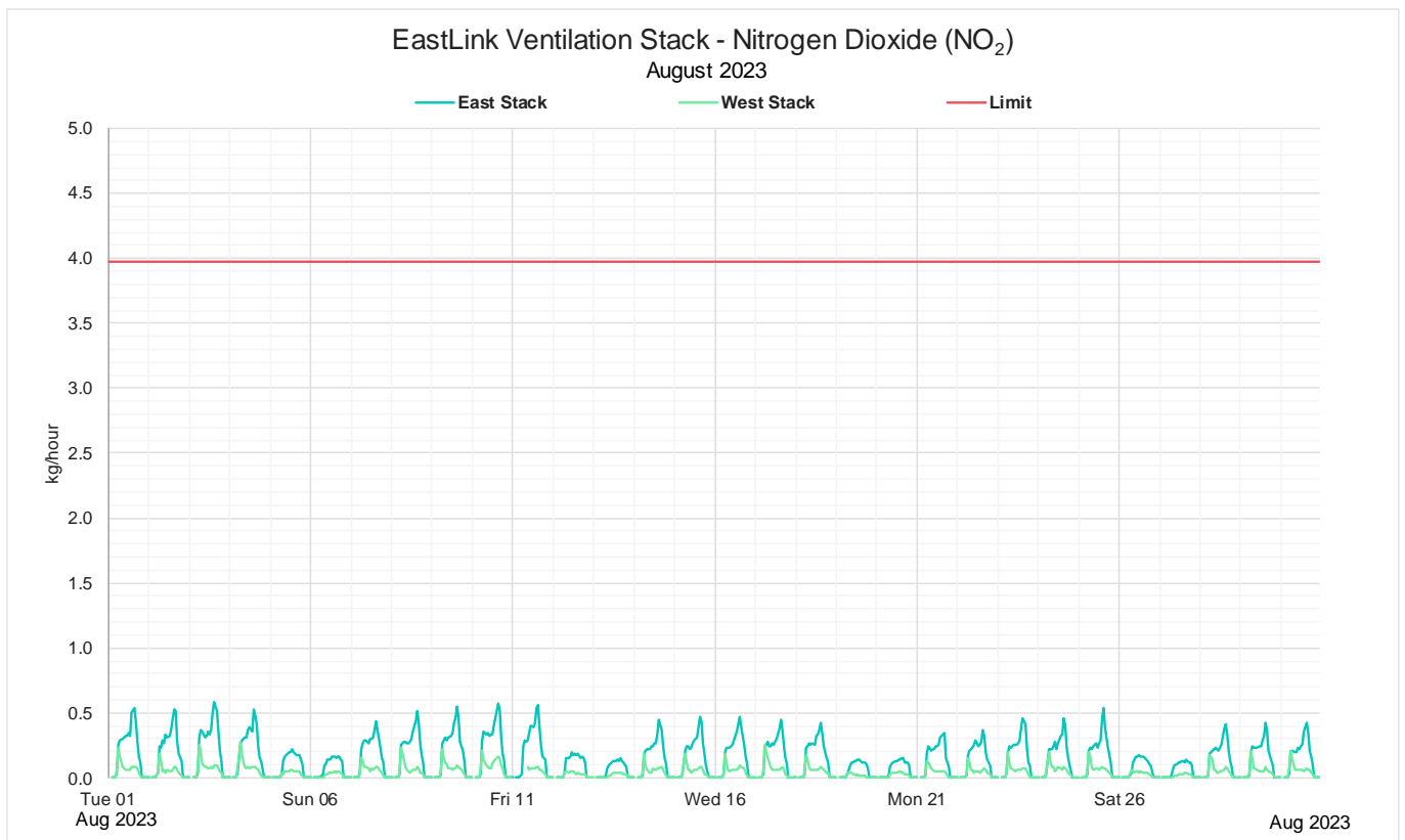
Figure 9: August 2023 Monthly 1 hour mass rate NO 2
