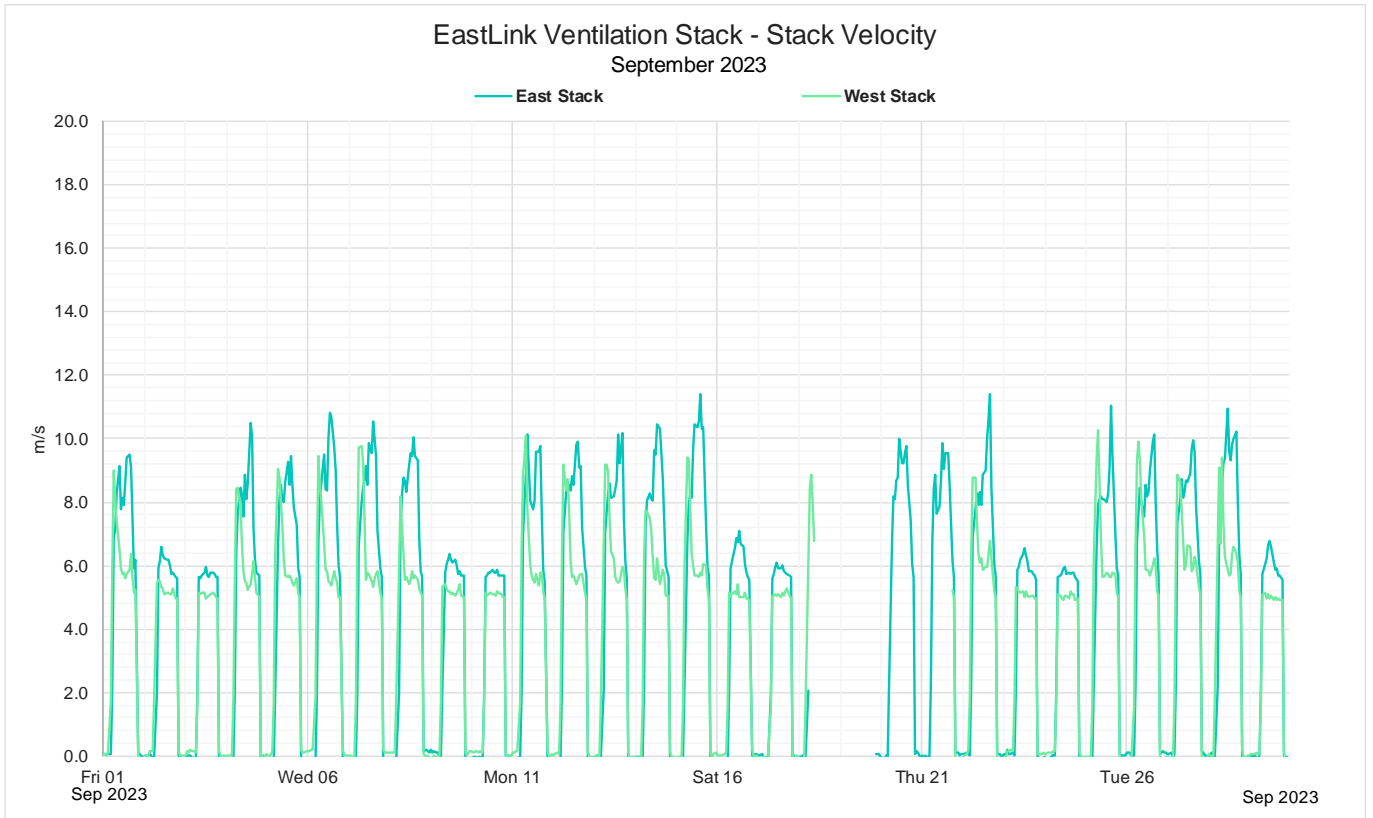
Figure 21: September 2023 Monthly 1 hour average stack velocity
