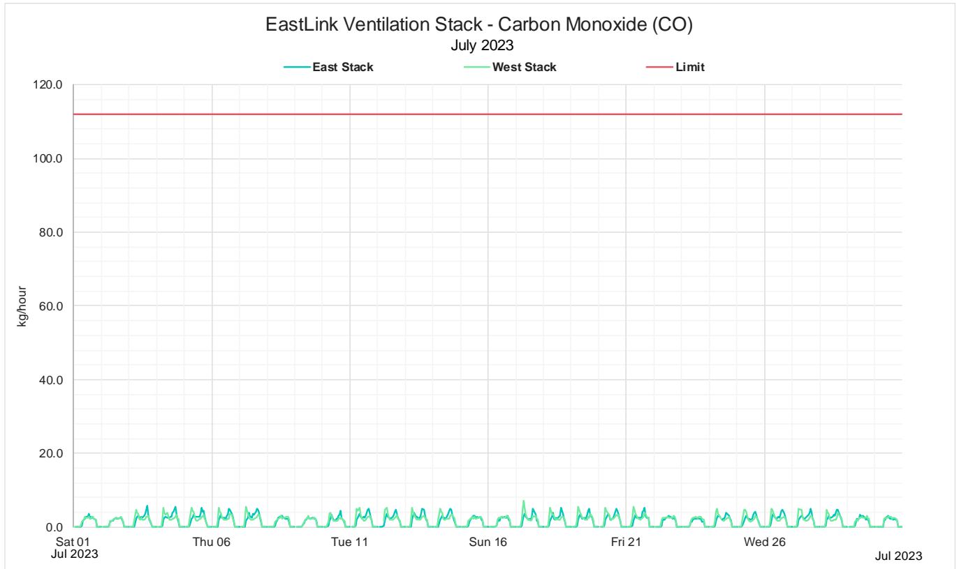
Figure 4: July 2023 Monthly 1 hour mass rate CO
