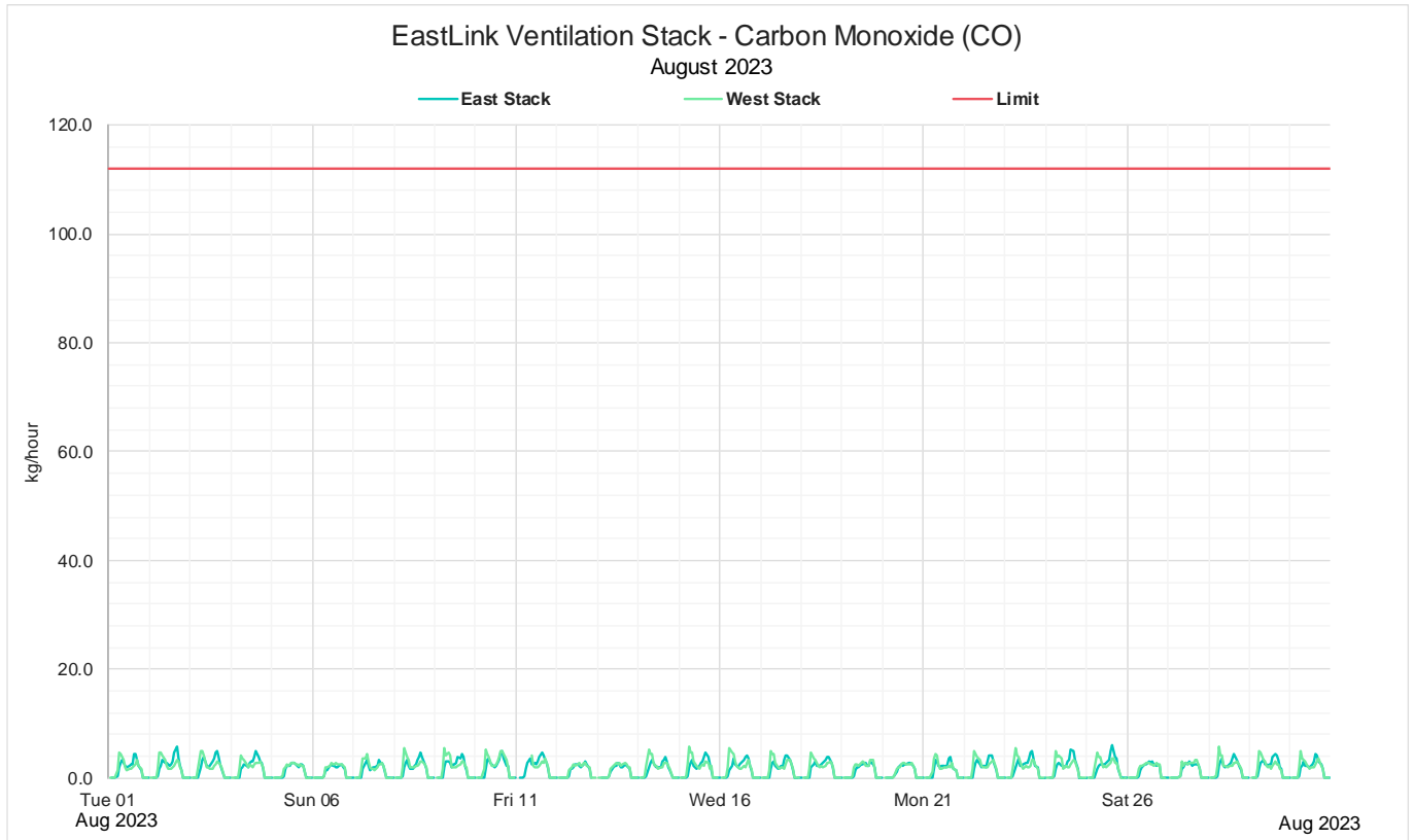
Figure 11: August 2023 Monthly 1 hour mass rate CO
