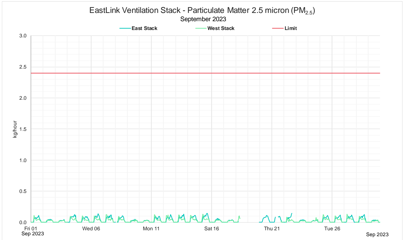
Figure 19: September 2023 Monthly 1 hour mass rate PM 2.5
