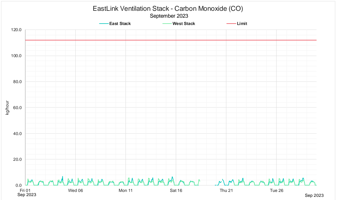
Figure 18: September 2023 Monthly 1 hour mass rate CO
