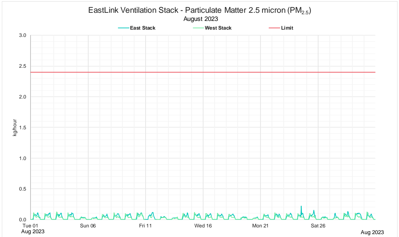
Figure 12: August 2023 Monthly 1 hour mass rate PM 2.5
