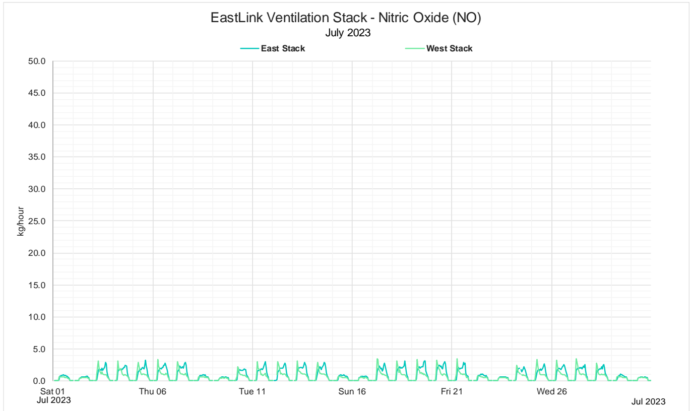
Figure 3: July 2023 Monthly 1 hour mass rate NO
