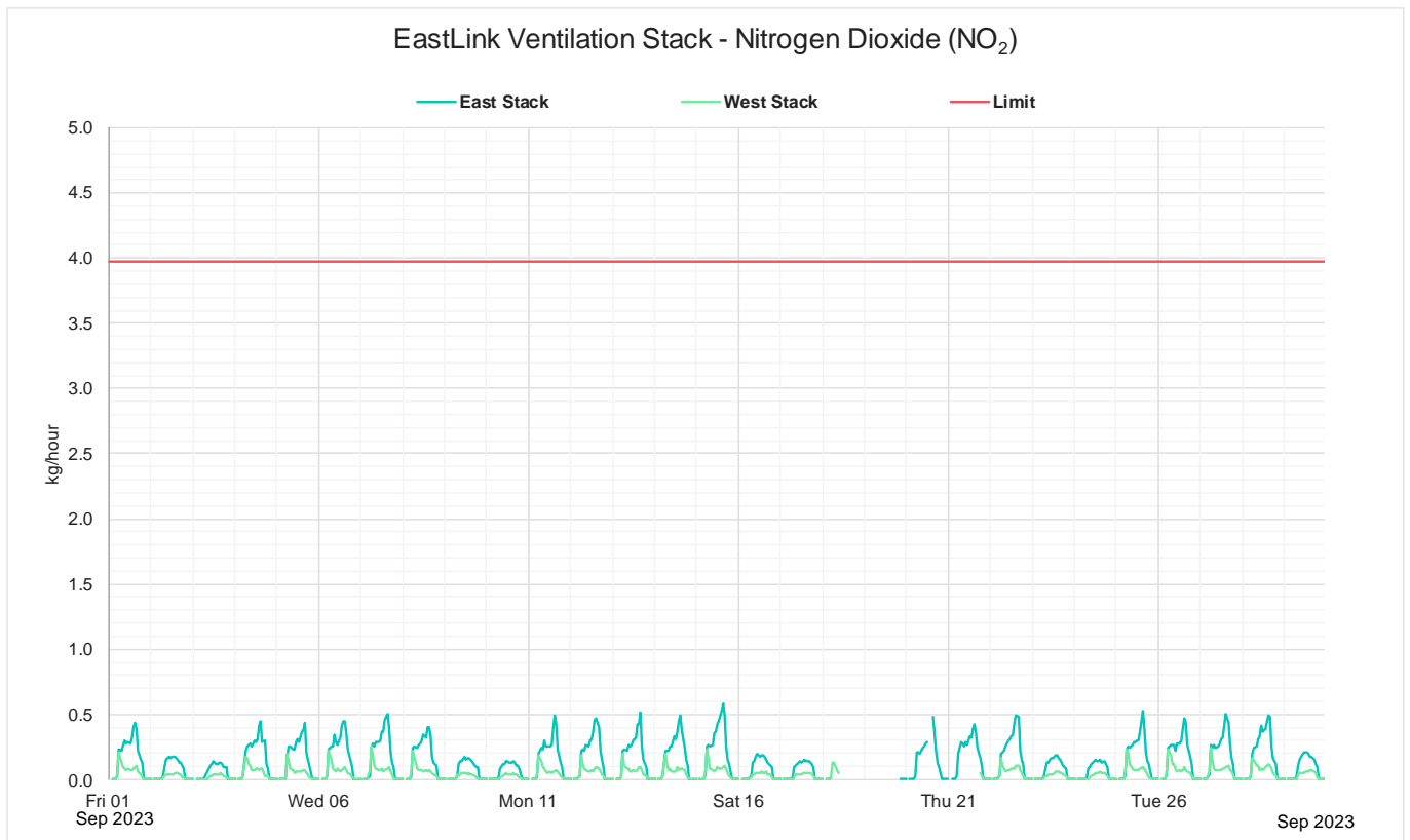
Figure 16: September 2023 Monthly 1 hour mass rate NO 2
