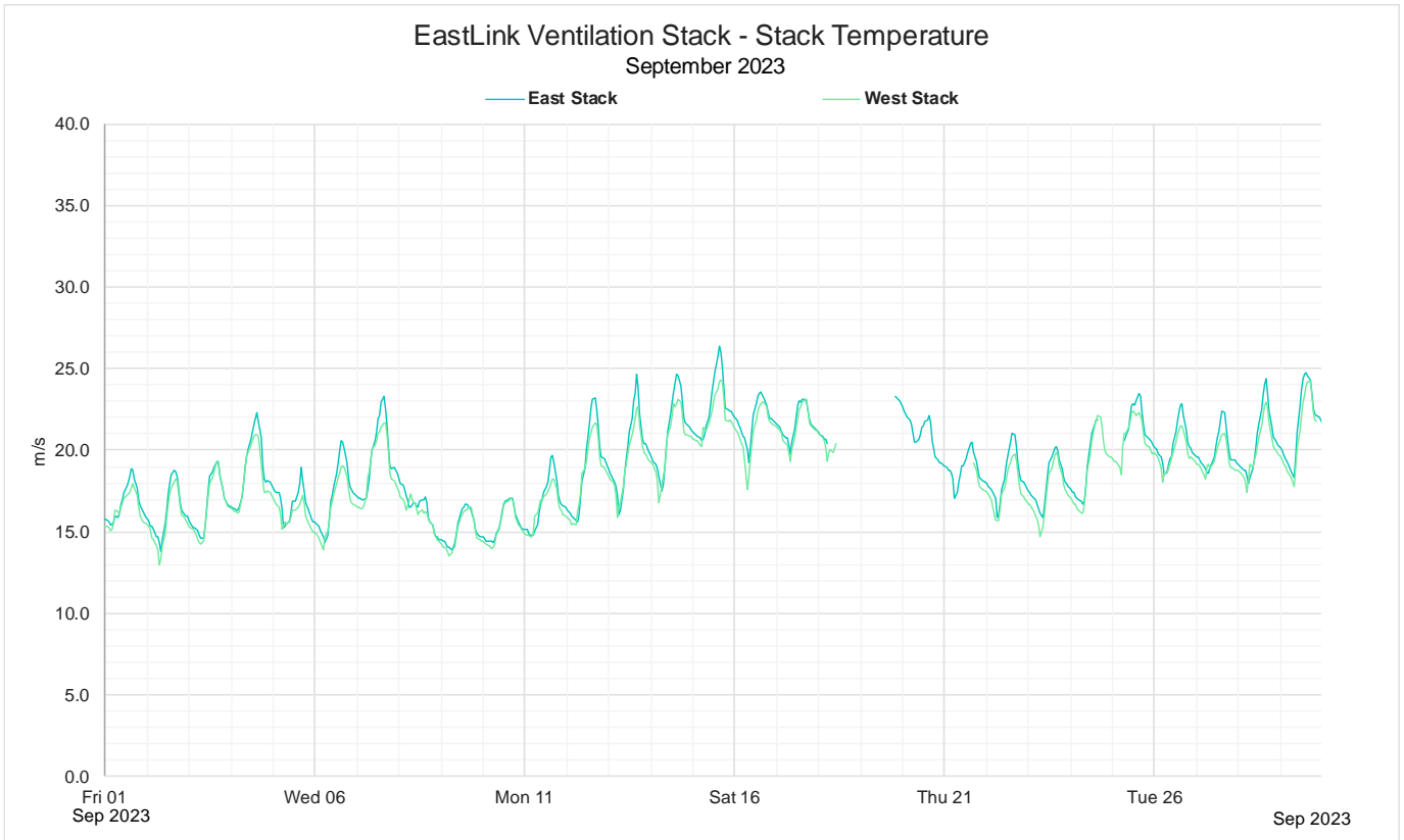
Figure 22: September 2023 Monthly 1 hour average stack temperature
