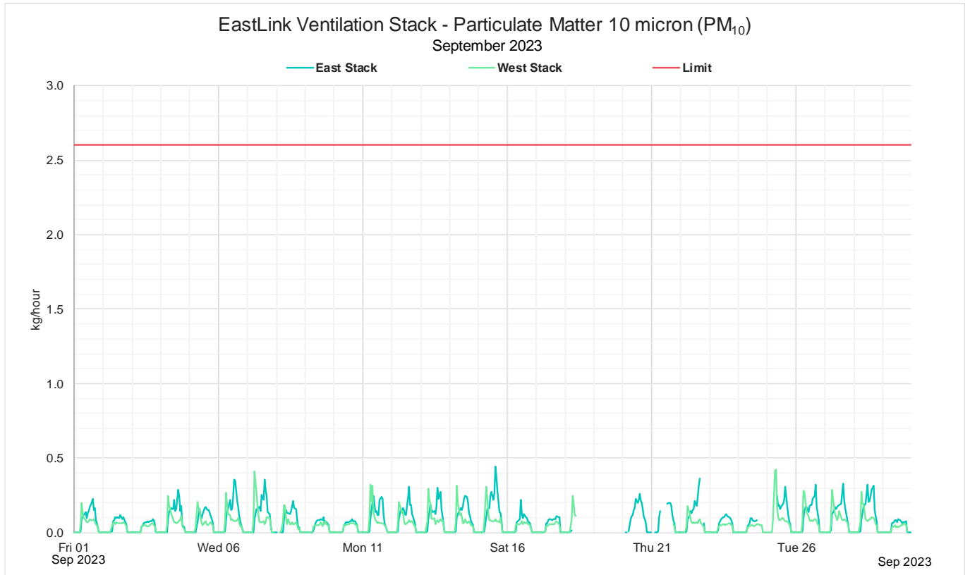
Figure 20: September 2023 Monthly 1 hour mass rate PM 10
