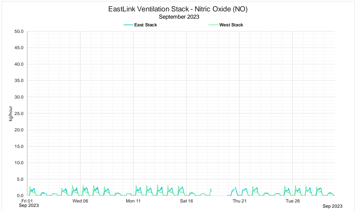
Figure 17: September 2023 Monthly 1 hour mass rate NO
