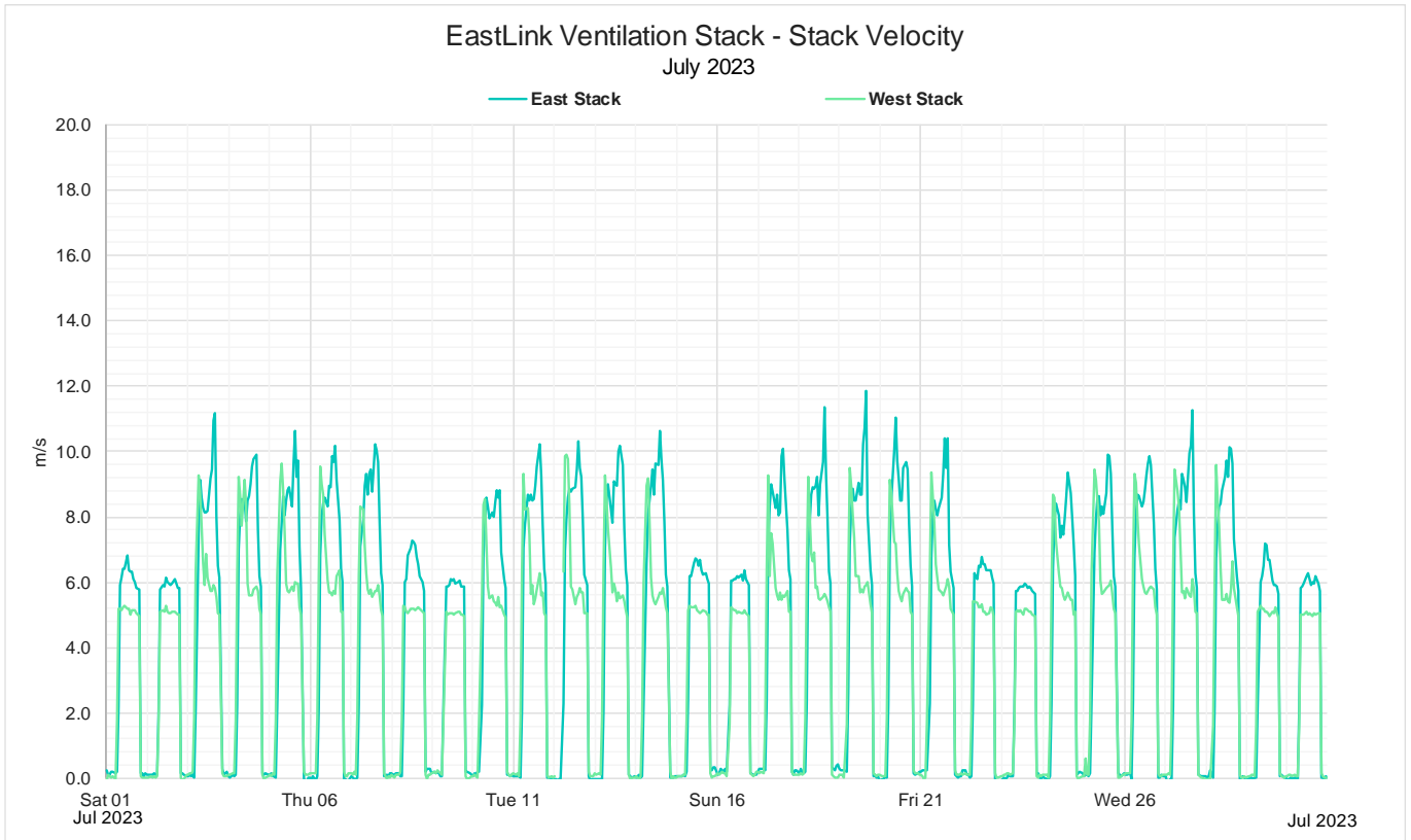
Figure 7: July 2023 Monthly 1 hour average stack velocity
