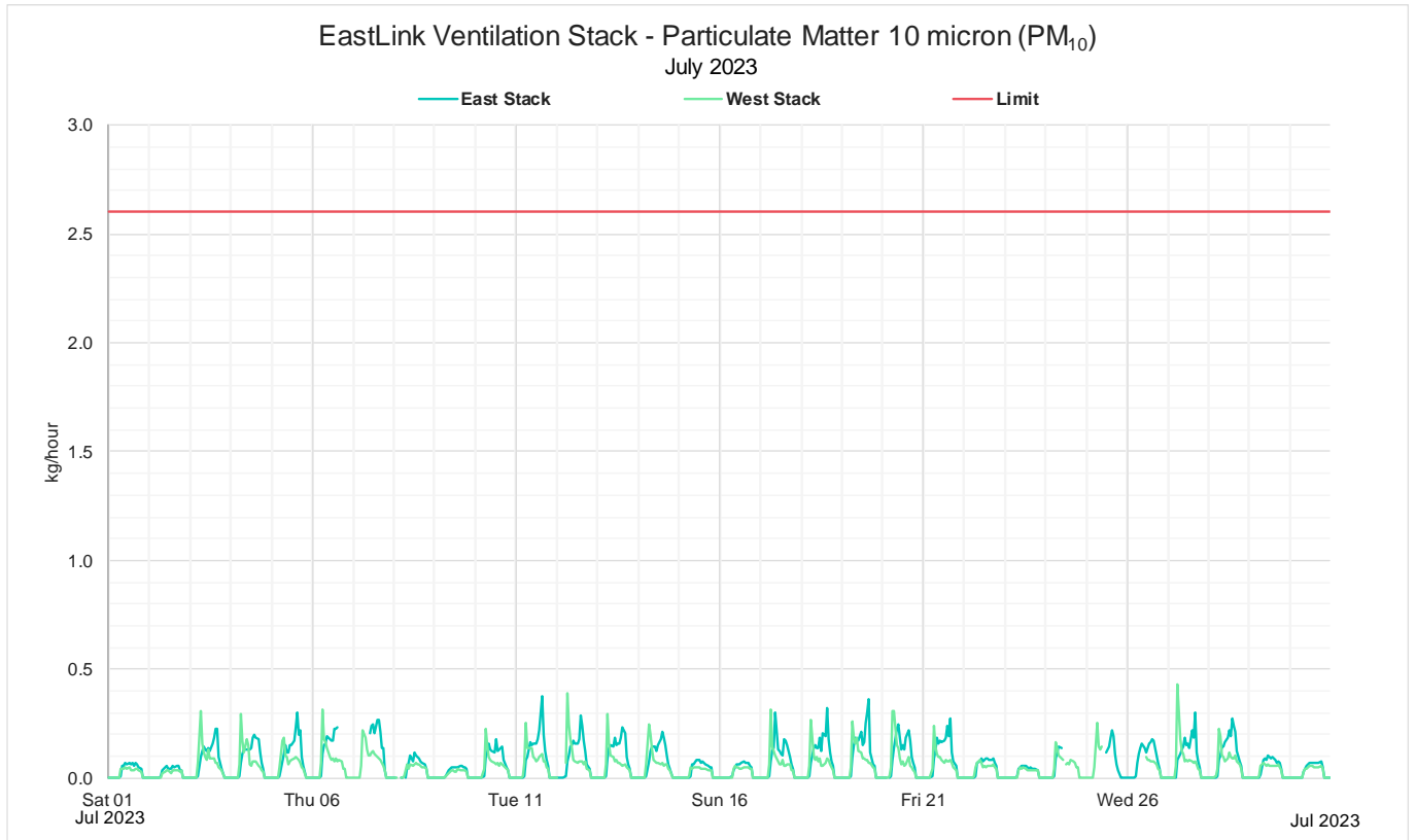
Figure 6: July 2023 Monthly 1 hour mass rate PM 10
