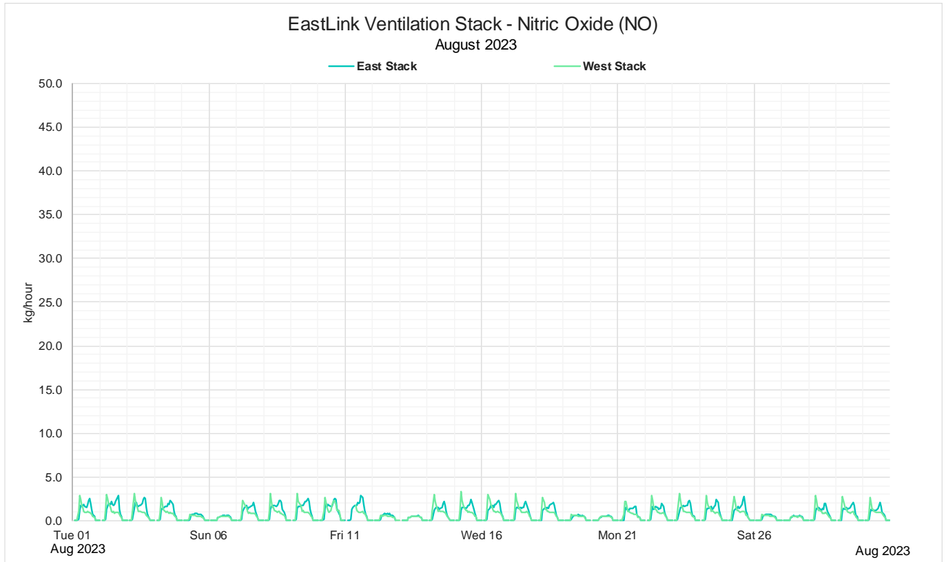
Figure 10: August 2023 Monthly 1 hour mass rate NO
