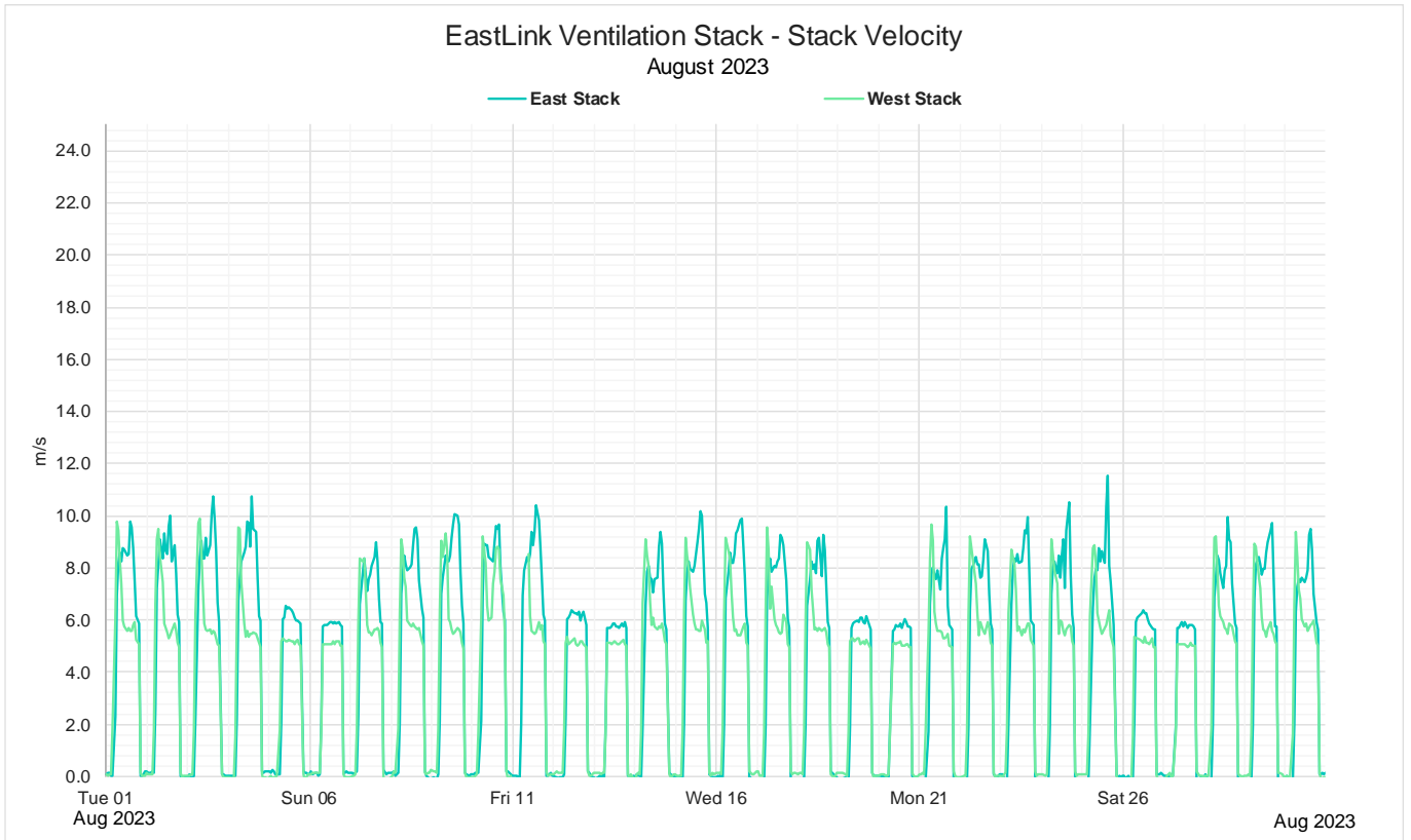
Figure 14: August 2023 Monthly 1 hour average stack velocity
